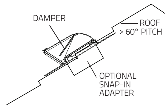
RVL28 - LOW PROFILE VENT
