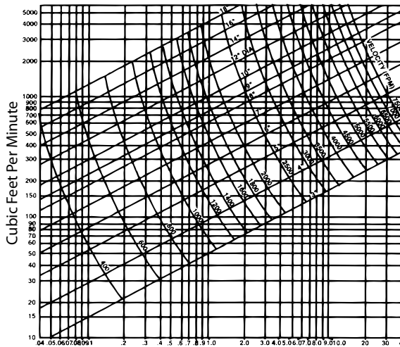
Friction Loss in inches of water per 100 ft.
