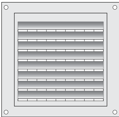
1/2" X 1/2" MOLDED FIXED LOUVER GRID ON FRONT OF VENT
