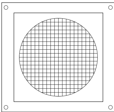
1/4" X 1/4" MOLDED GRID ON INSIDE FRAME 5" THRU 8" ONLY
