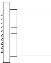
1/2" X 1/2" MOLDED FIXED LOUVER GRID ON FRONT OF VENT 5" THRU 8" ONLY
