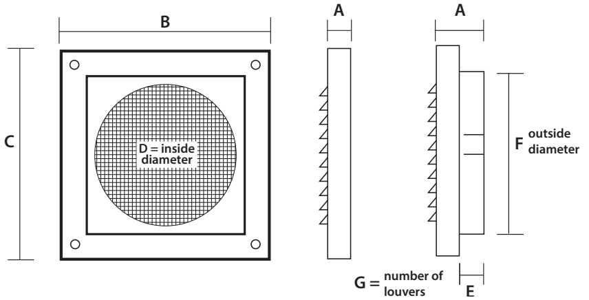
1/4" X 1/4" MOLDED FIXED LOUVER GRID ON FRONT OF VENT
